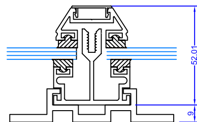
Fixing Cleat Shoe
