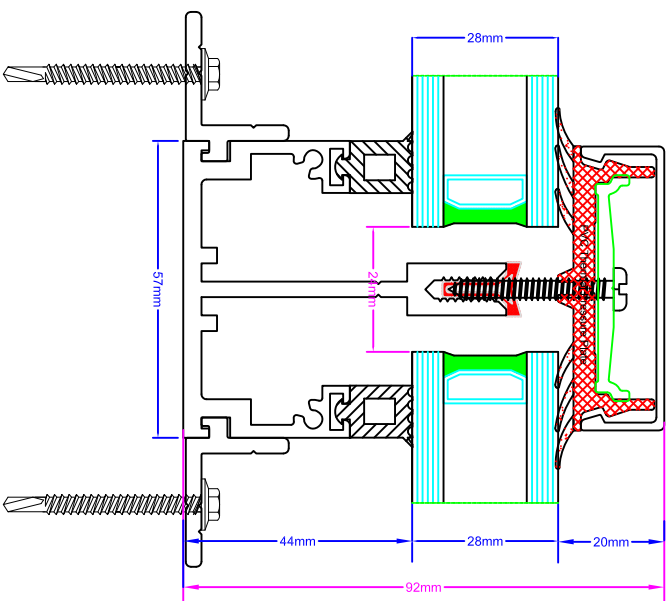
Centre Bar
