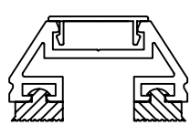
Sloping cap
