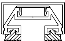
Square cap
