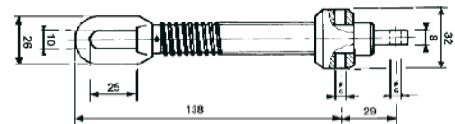
TELESCOPIC SPINDLE
